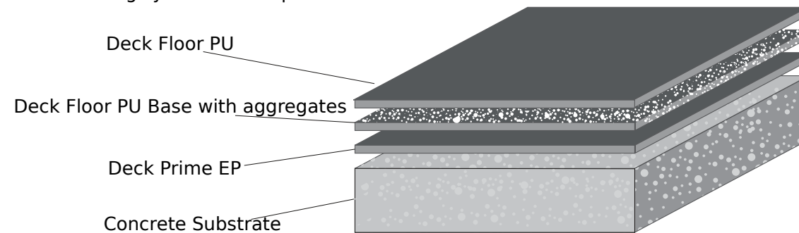
Figure 1: Schematic for Deck Floor PU System
